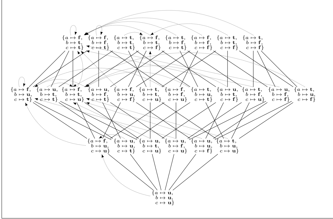
Figure 3: Complete meet-semilattice of three-valued interpretations over S_1 = \{a, b, c\} under the information ordering for Example 15; dotted arrows visualise mappings of the operator \Gamma_{D_1} . It can be seen that \Gamma_{D_1} has a \leq_i -least fixpoint, which is situated right \leq_i -beneath its two-valued models, the other two fixpoints of \Gamma_{D_1} .
