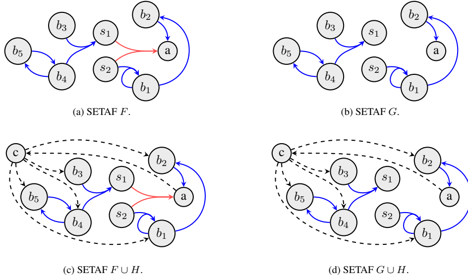
Figure 15: Example of two SETAFs F and G which disagree on their kernels (witnessed by the attack (\{s_1, s_2\}, a) colored in red) but \text{com}(F) = \text{com}(G) and the extended SETAFs F \cup H, G \cup H where \text{com}(F \cup H) \neq \text{com}(G \cup H) holds.
