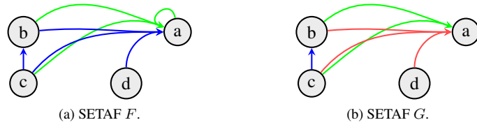
Figure 3: Example of a reducible attack (in SETAF F , colored in green) and the framework which arises after replacement (SETAF G , attack in red becomes redundant).
