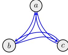
Figure 1: An example SETAF with three collective attacks.
