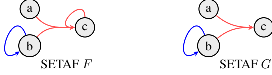
Figure 10: Given that (\{a, b\}, c) is inactive it is equivalent to (\{a, b, c\}, c) for all semantics under our considerations. We call the attack (\{a, b, c\}, c) in F reducible and G the normal form of F .
