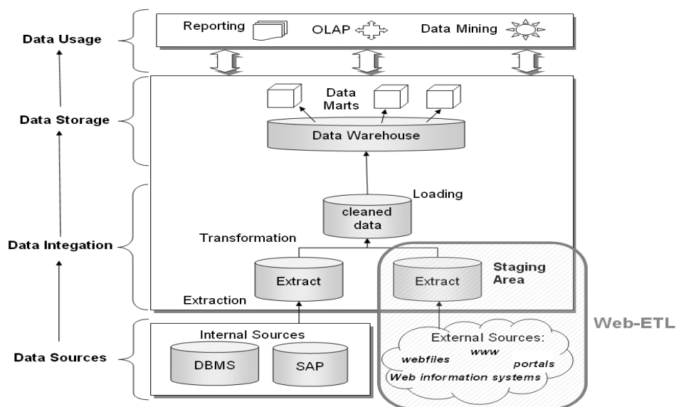
Figure 1: The Business Intelligence reference process.
