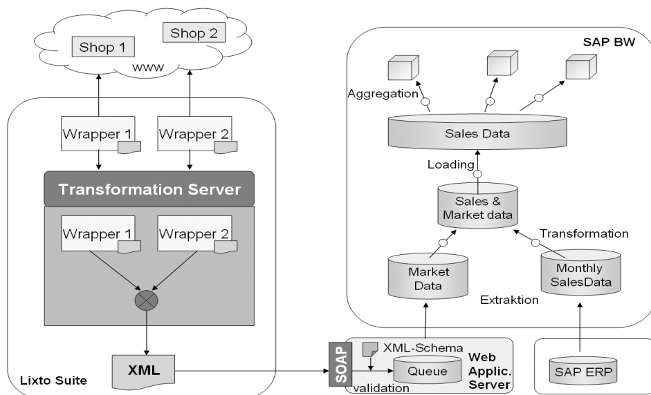
Figure 6: The data extraction and the BI integration process.
