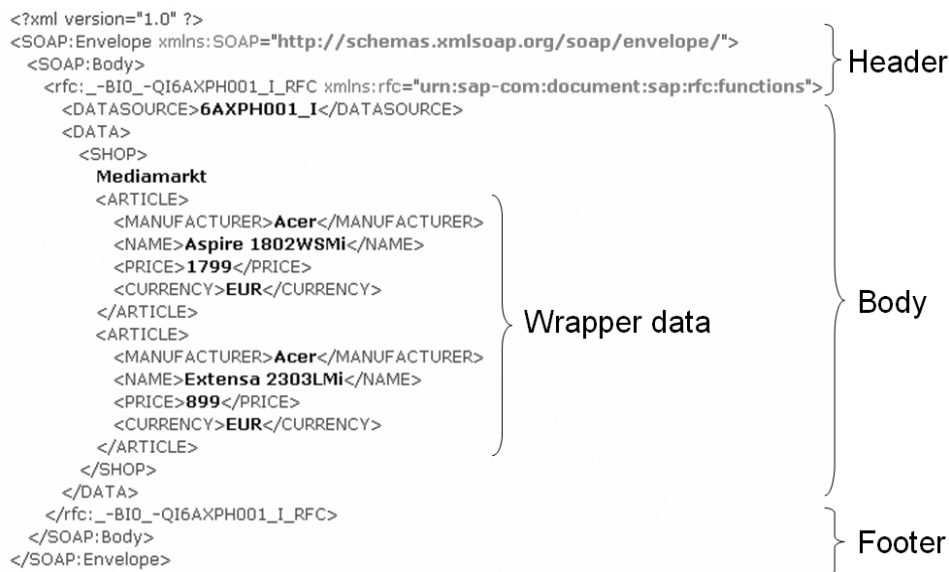
Figure 5: SOAP message with wrapper data.
