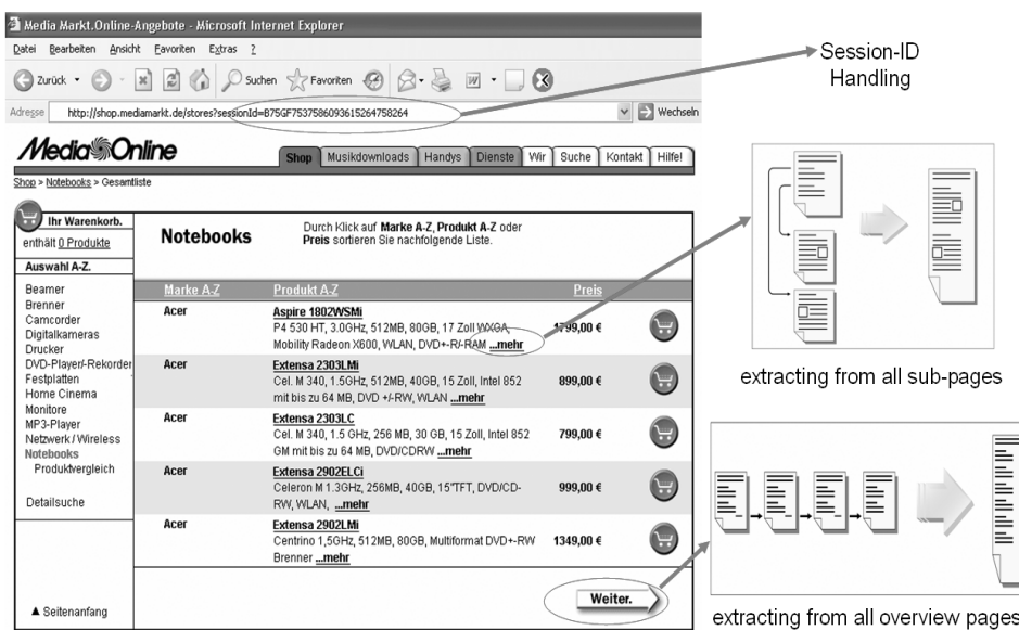
Figure 3: Extraction of all article data.
