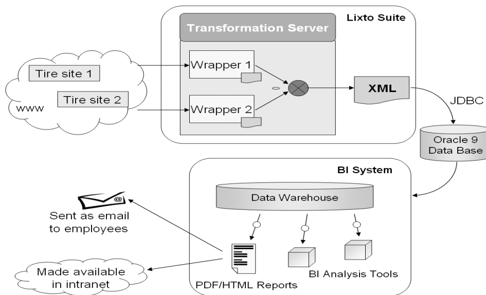
Figure 8: System structure overview.
